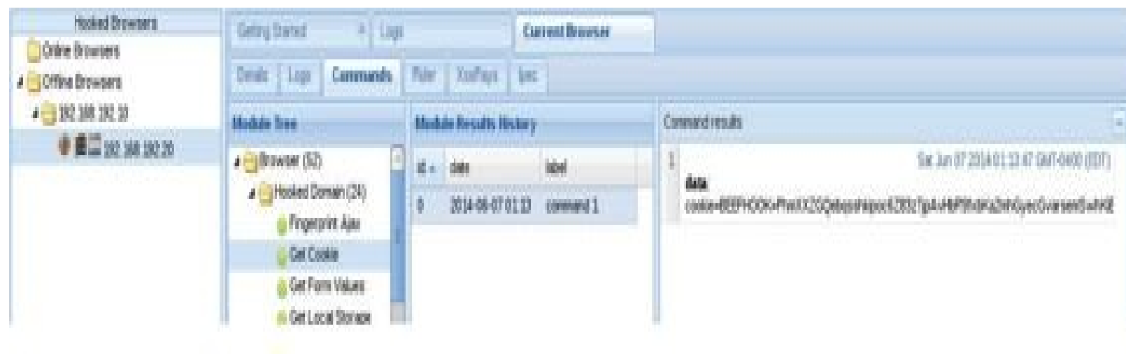
Figure 18-18 Viewing cookies retrieved using Autorun
