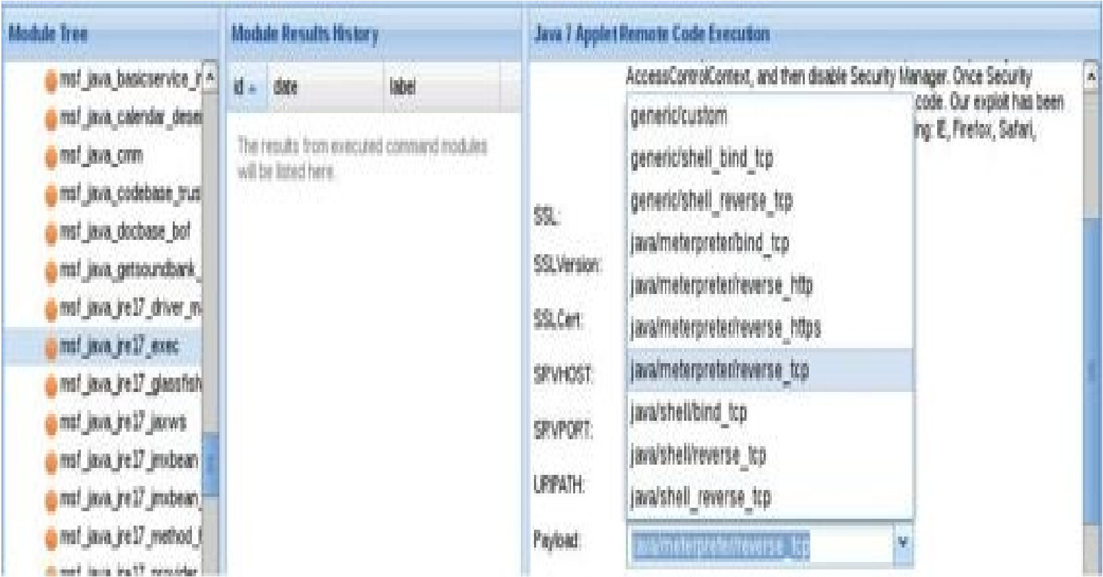
Figure 18-15 The Java 7 Applet Remote Code Execution Metasploit module in BeEF
