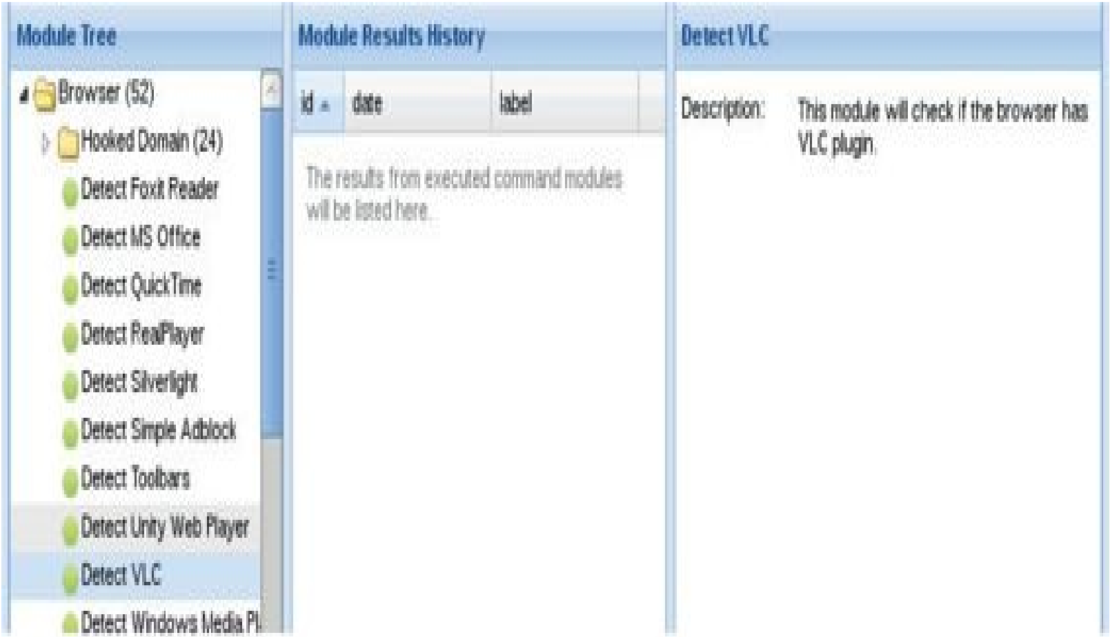
Figure 18-8 Selecting the VLC plug-in check
