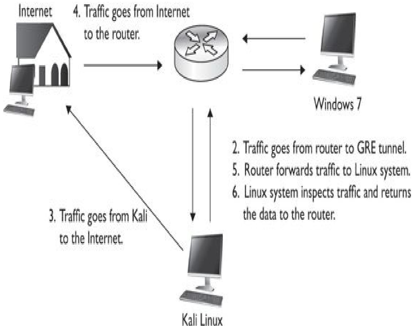
Figure 9-3 The final GRE tunnel workflow
