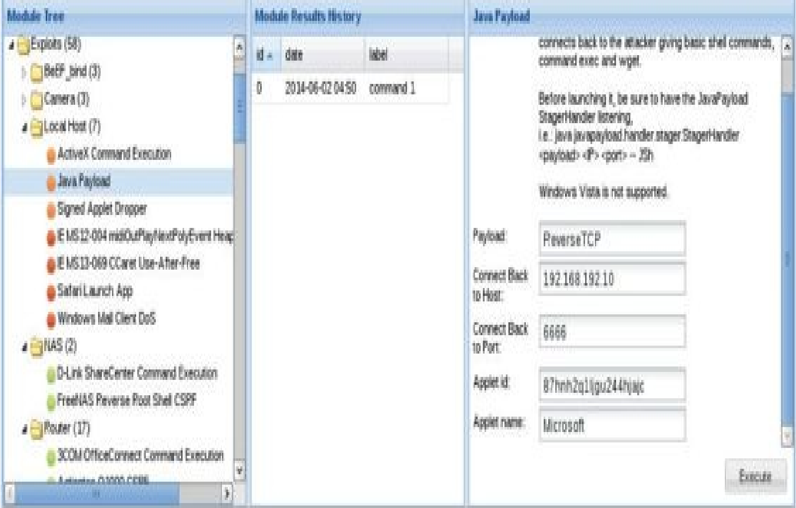
Figure 18-14 The module settings for the Java Payload module
