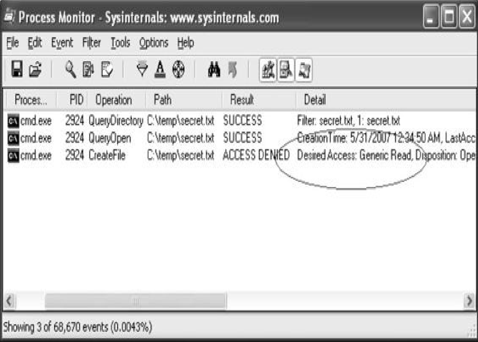
Figure 14-20 Process Monitor log of type c:\temp\secret.txt
