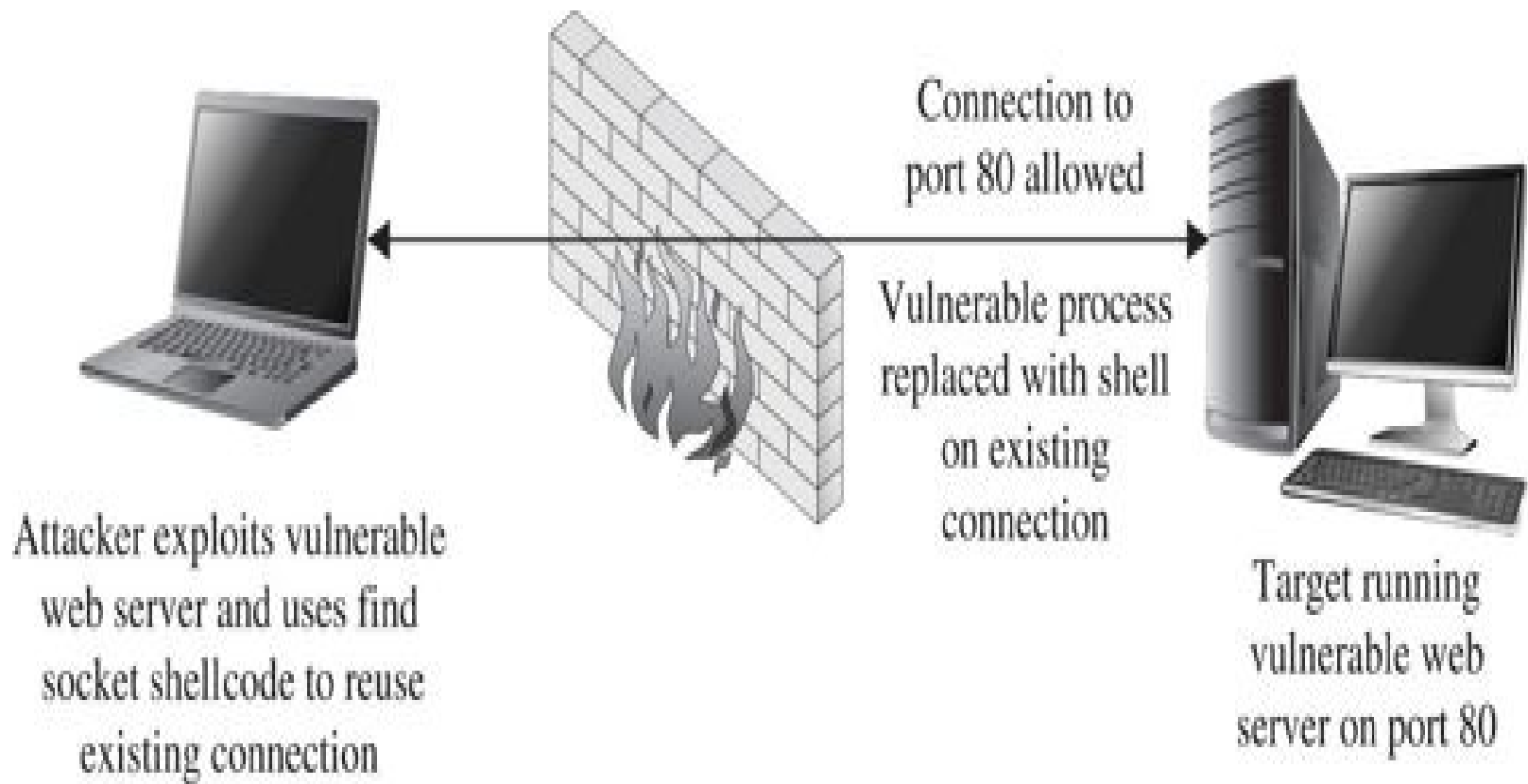
Figure 6-5 Network conditions suited for find socket shellcode
