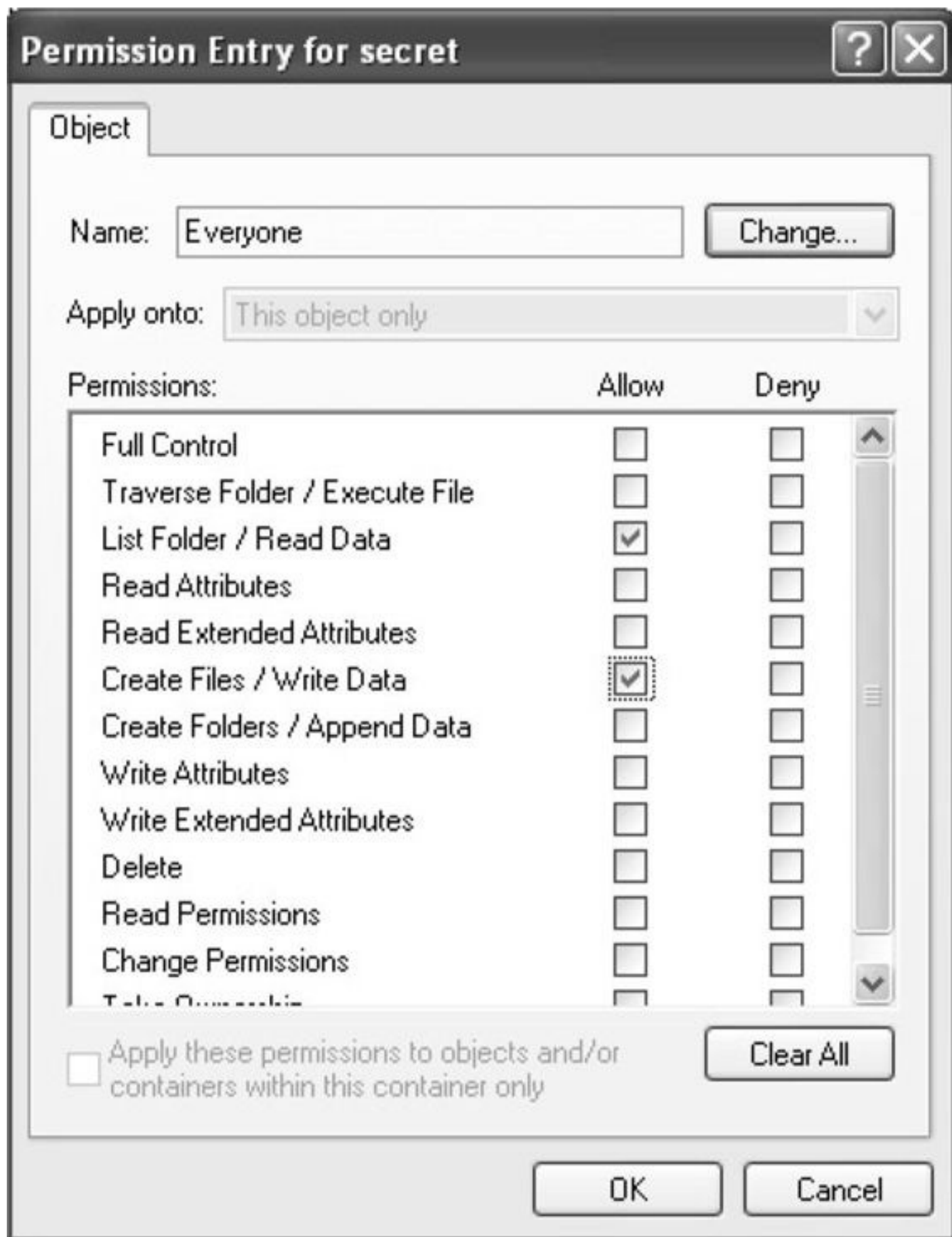
Figure 14-17 Windows permissions display for c:\temp\secret.txt
