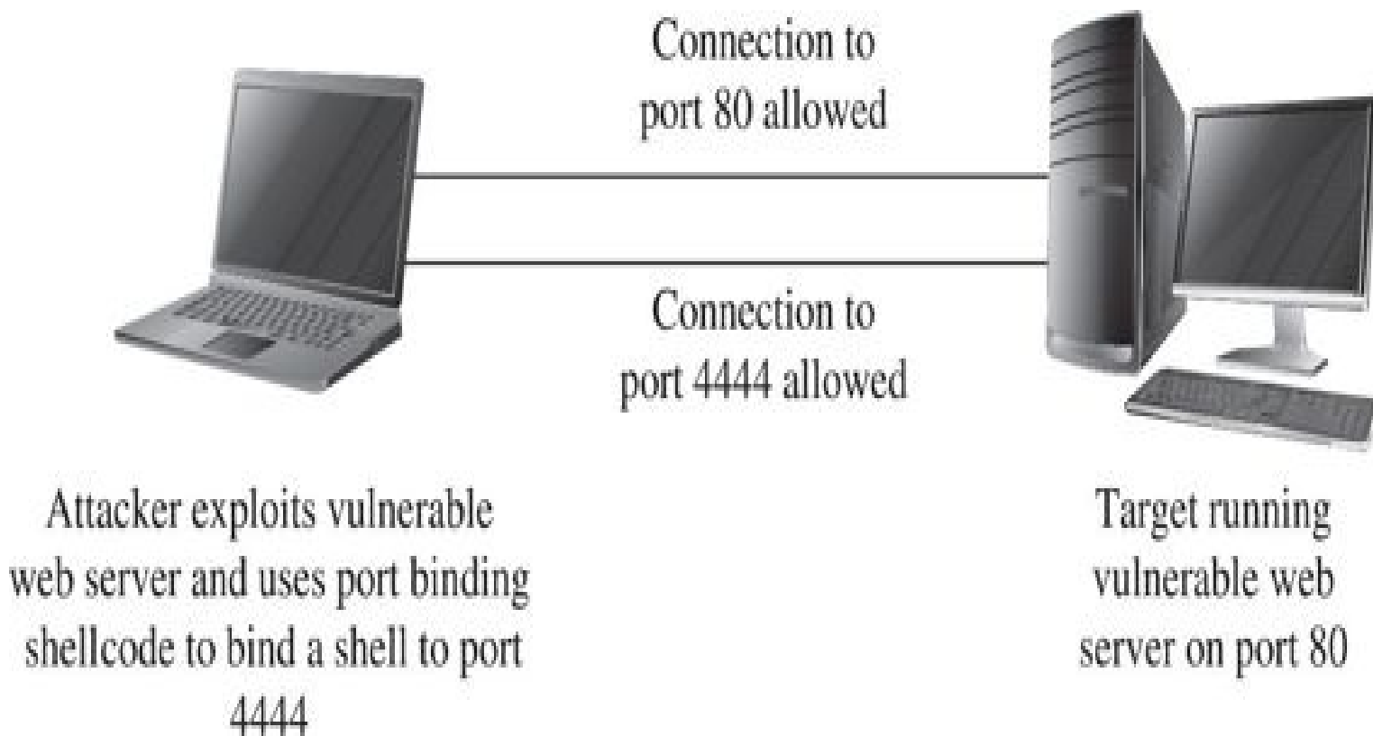
Figure 6-1 Network layout that permits port binding shellcode
