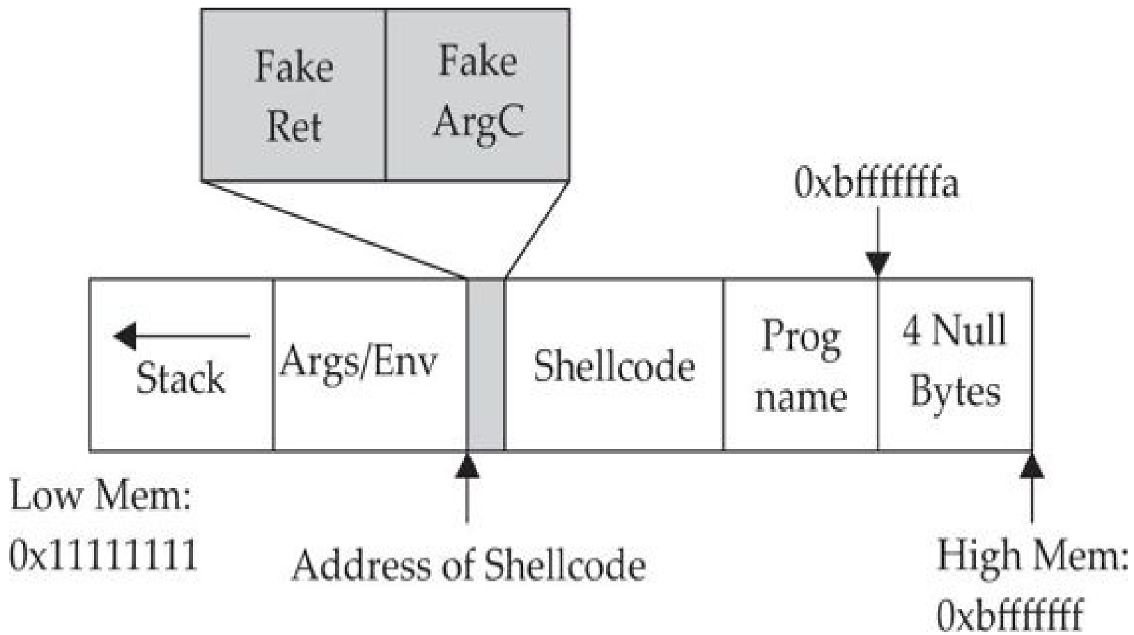
Figure 11-3 Using a fake frame to attack small buffers
