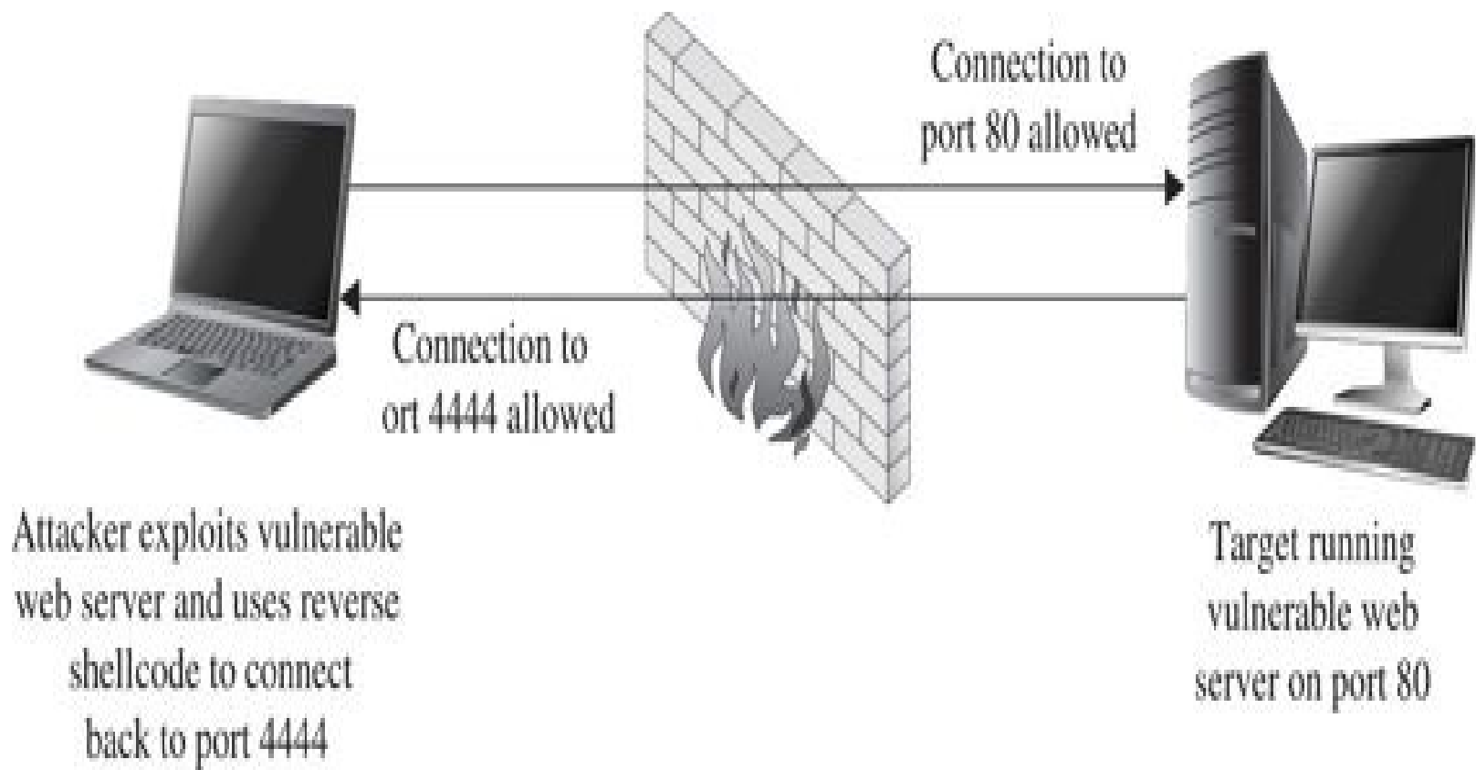
Figure 6-3 Network layout that facilitates reverse connecting shellcode
