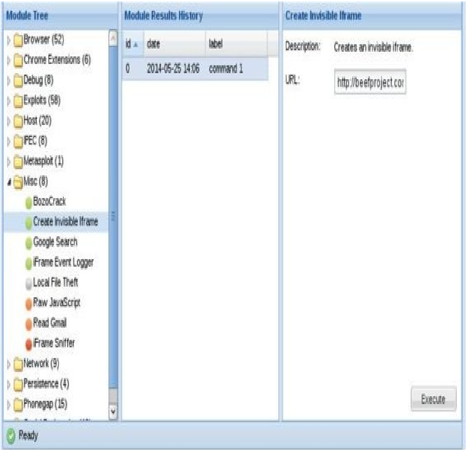
Figure 18-4 The Commands tab display
