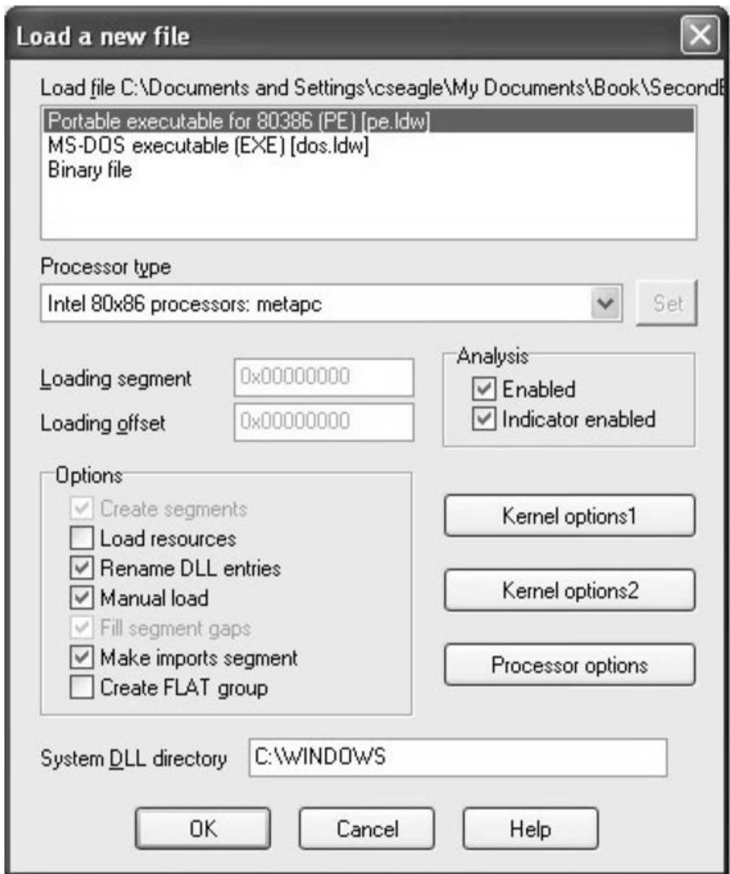
Figure 4-3 Forcing a manual load with IDA Pro
