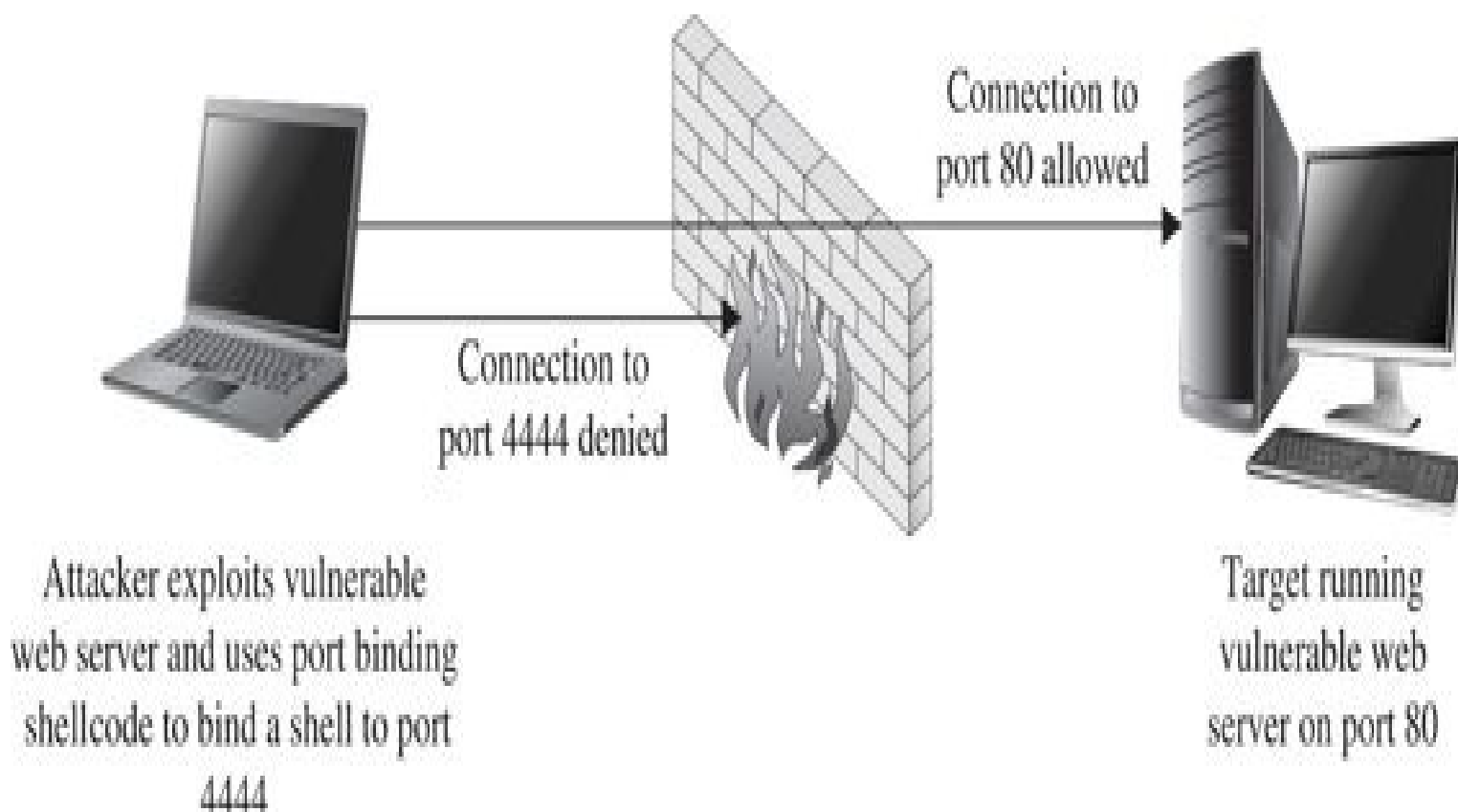
Figure 6-2 Firewall configured to block port binding shellcode
