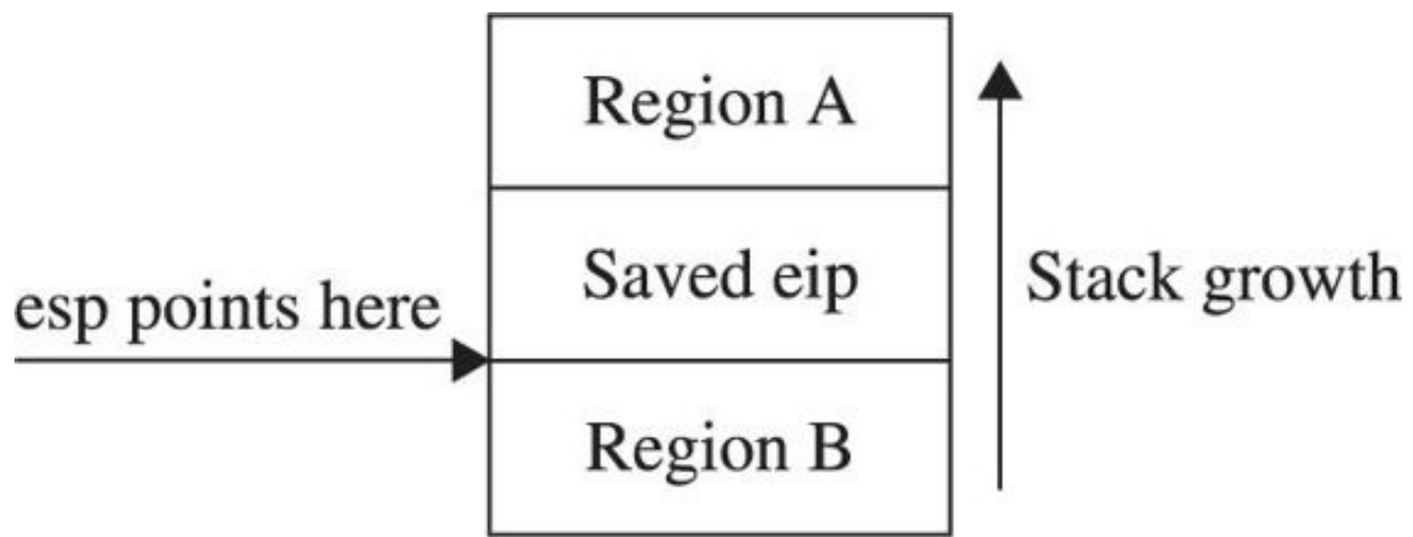
Figure 6-8 Shellcode layout in a stack overflow
