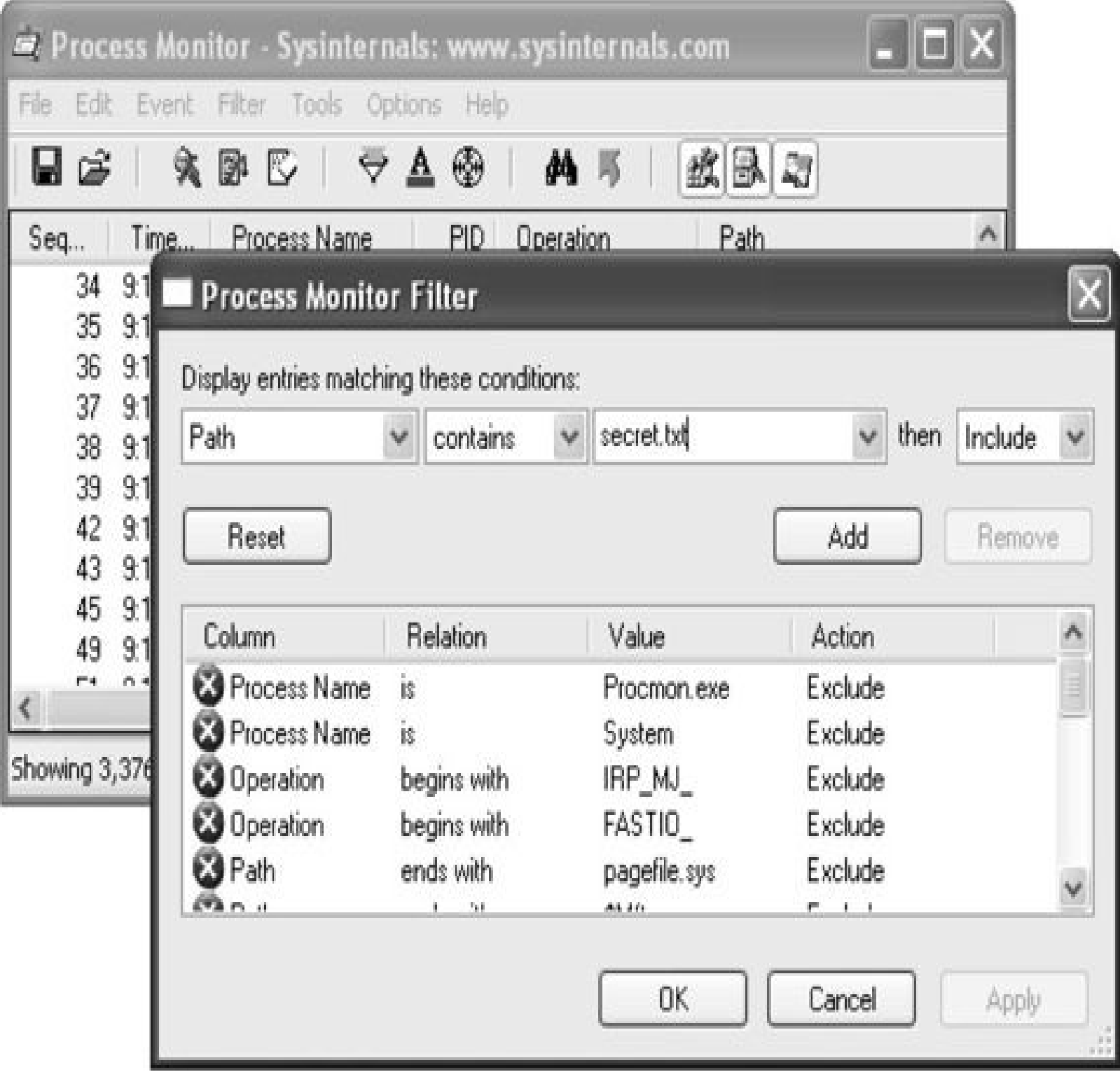
Figure 14-19 Building a Process Monitor filter
