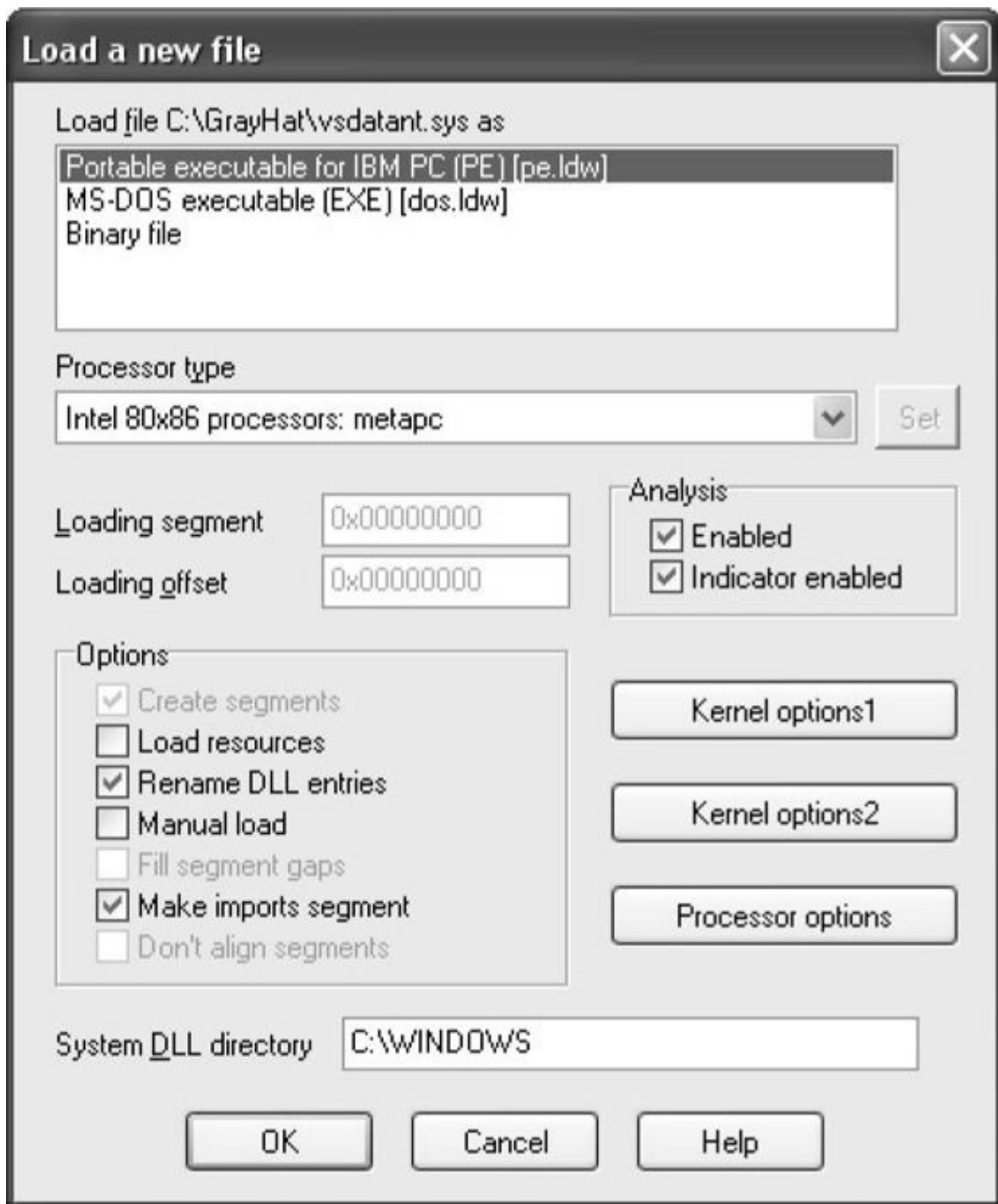
Figure 3-1 The IDA Pro file upload dialog
