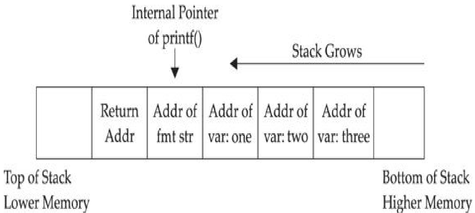
Figure 11-1 Depiction of the stack when printf() is executed
