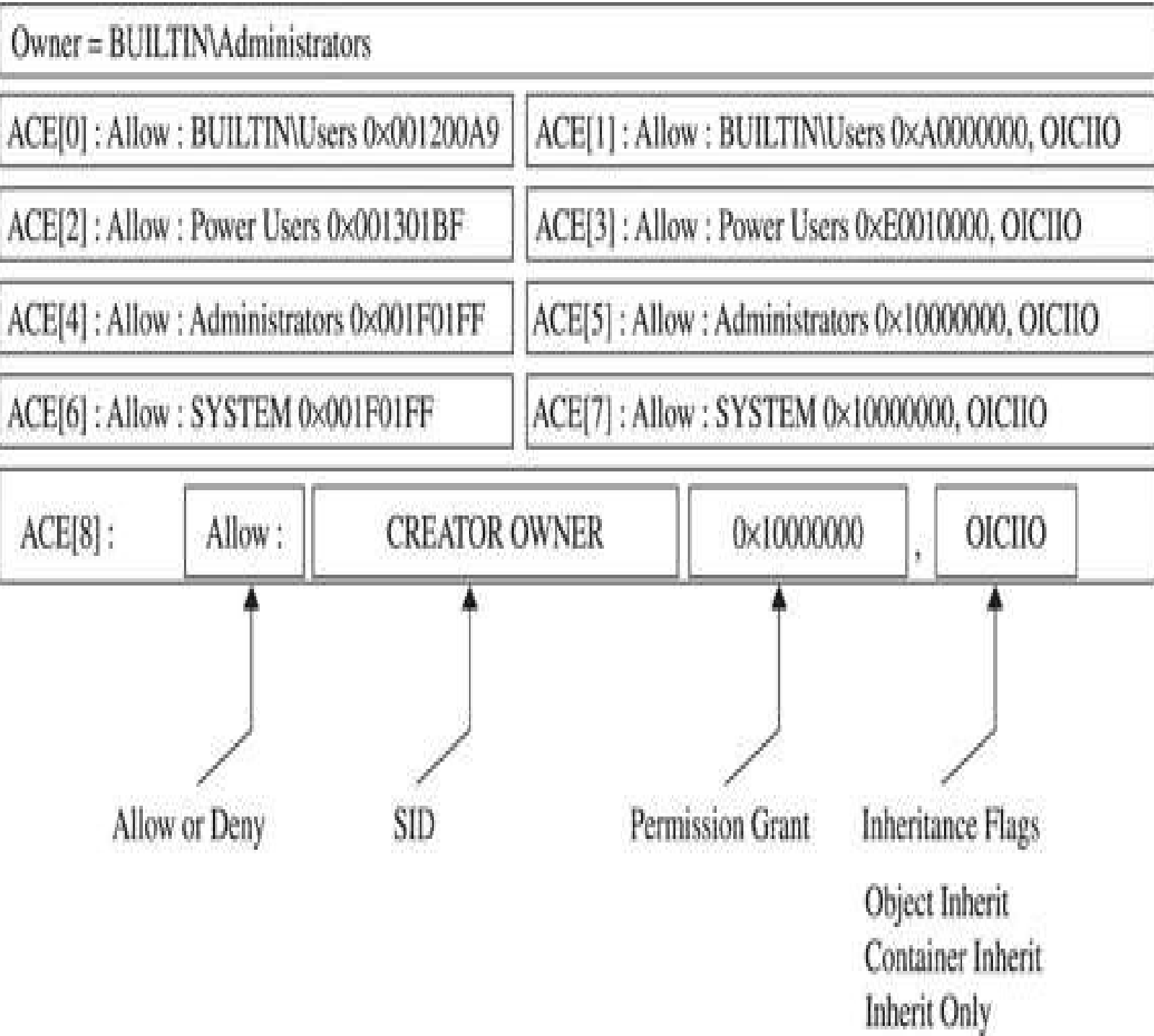
Figure 14-4 C:\Program Files security descriptor
