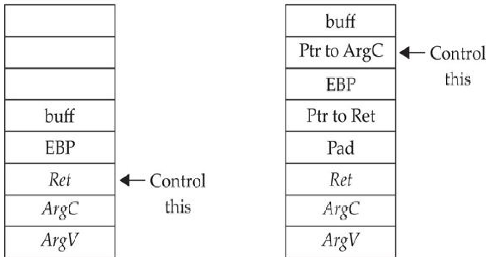
Figure 11-2 Old and new prolog
