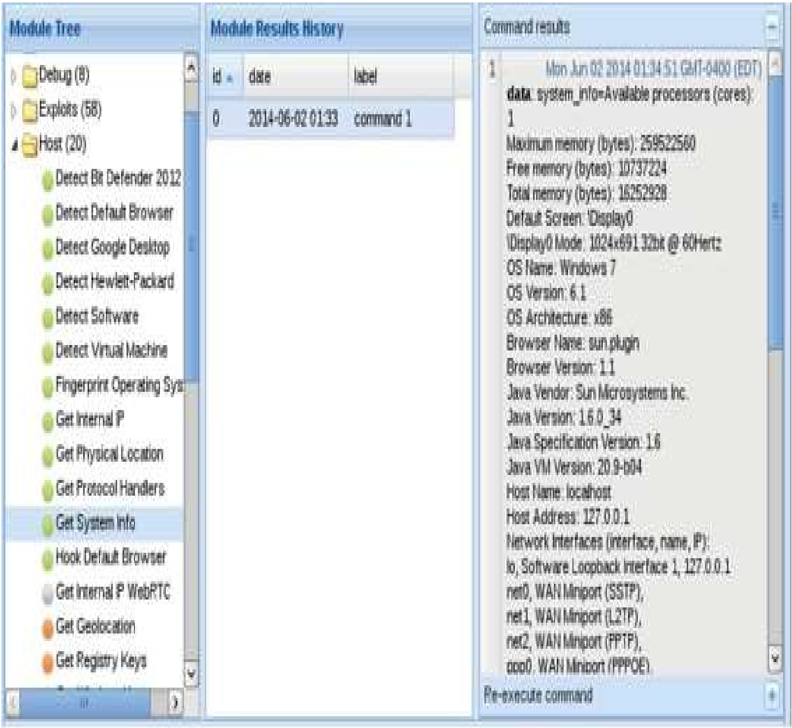
Figure 18-12 The output from the Get System Info module
