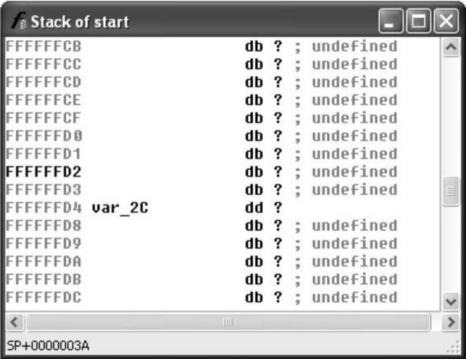
Figure 3-4 IDA Pro stack frame prior to type consolidation
