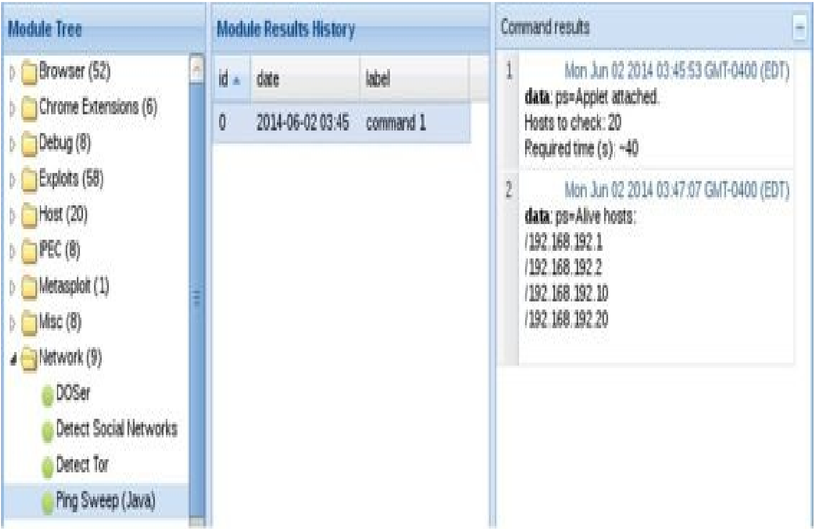
Figure 18-13 The output from the Ping Sweep module
