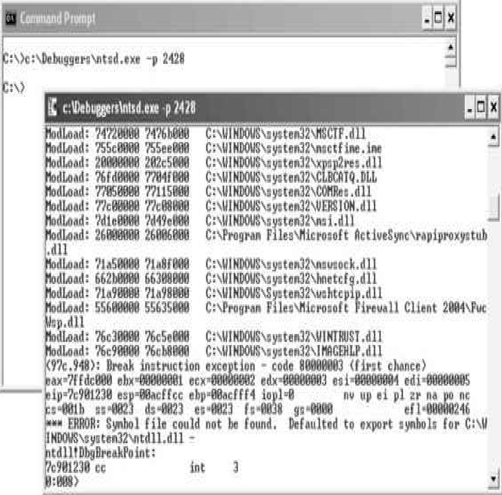
Figure 14-10 Windows debugger
