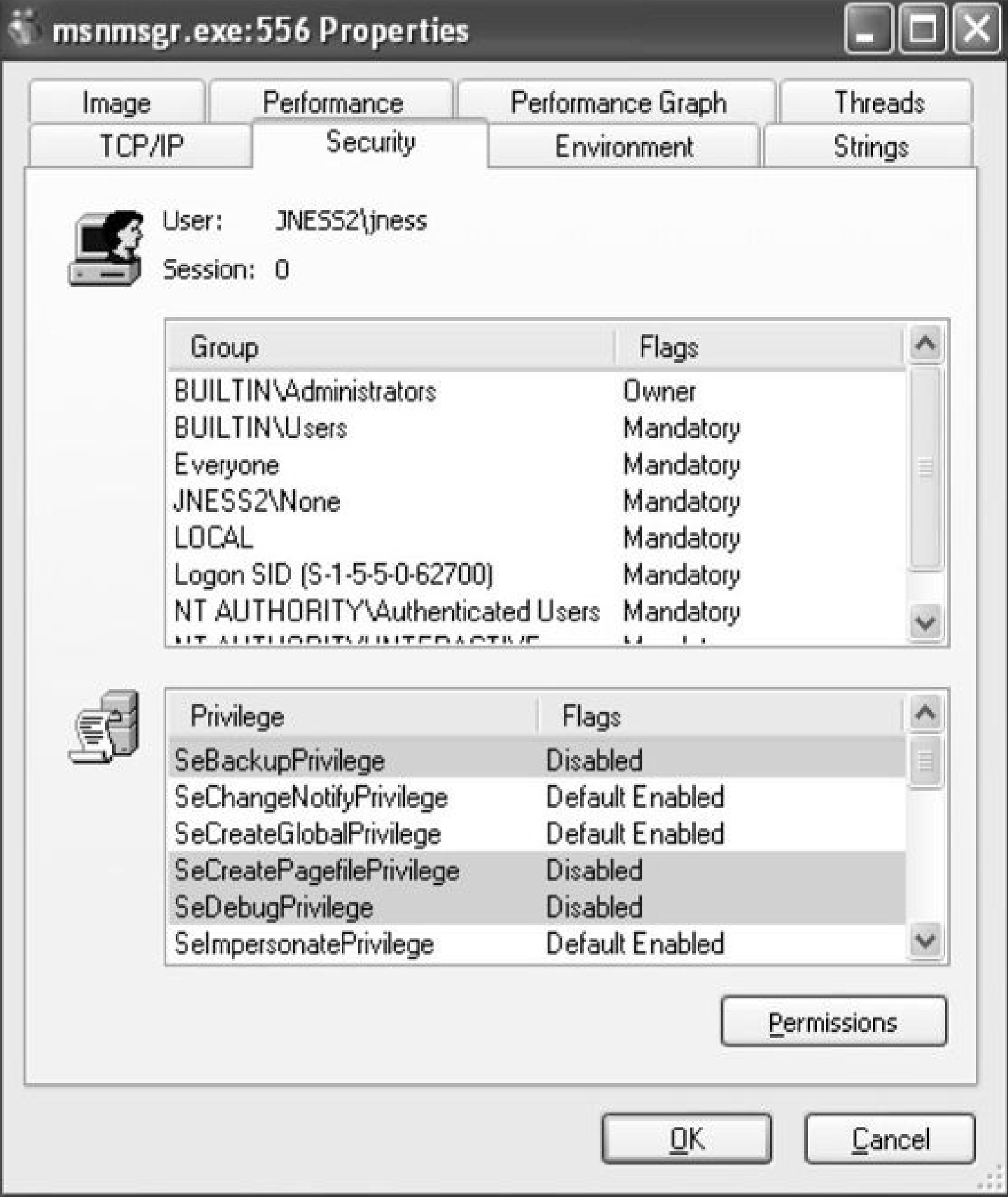
Figure 14-1 Process token
