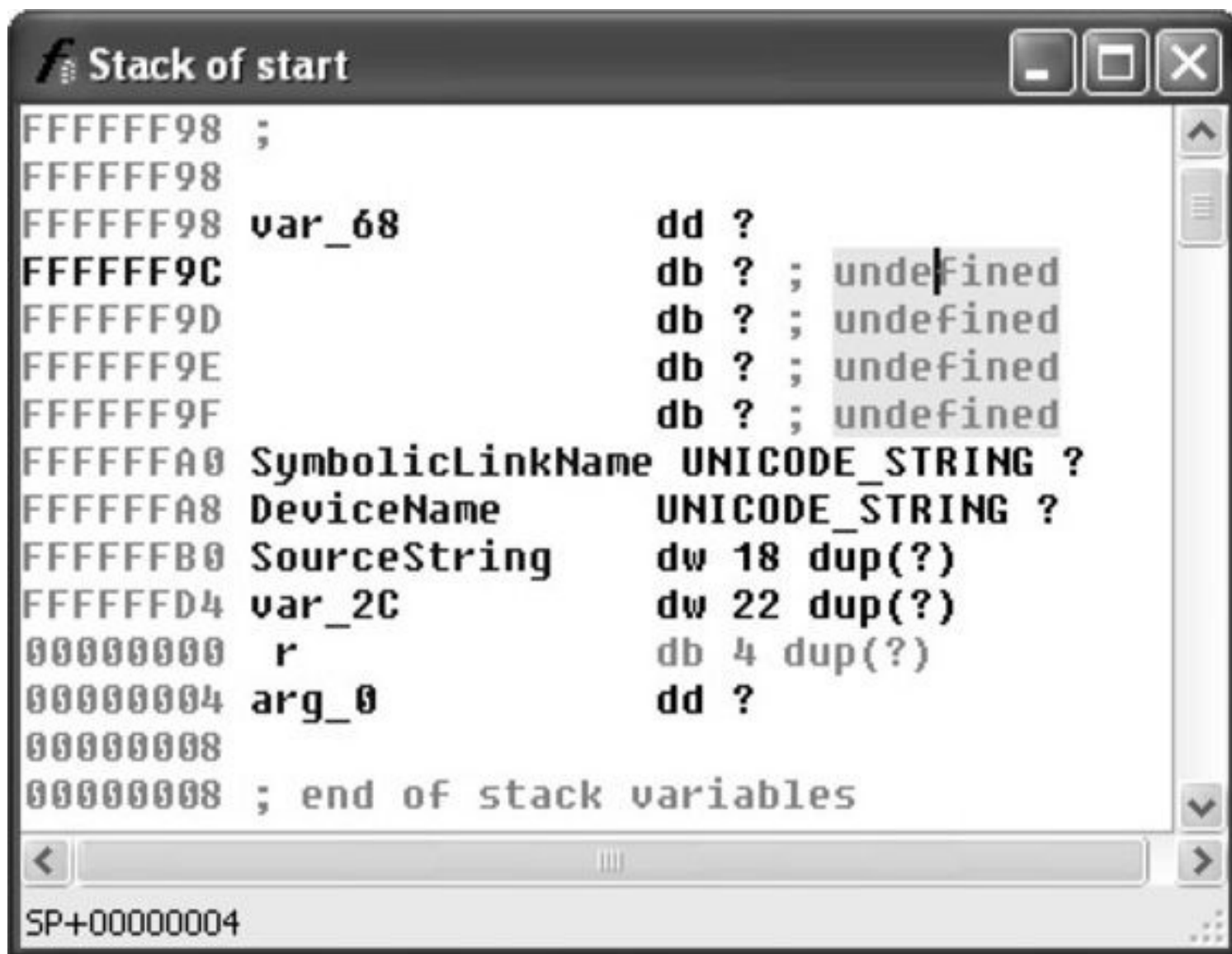
Figure 3-5 IDA Pro stack frame after type consolidation
