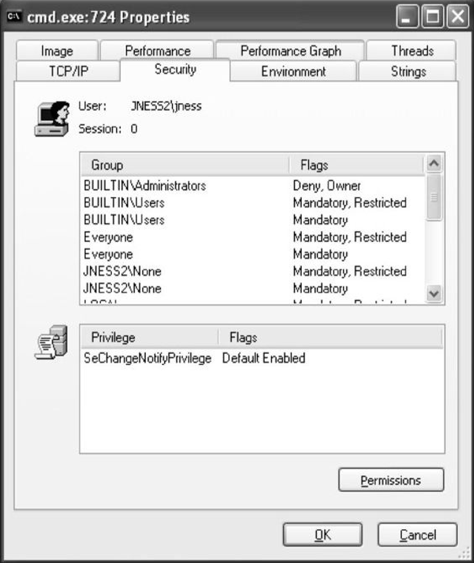
Figure 14-3 Restricted token
