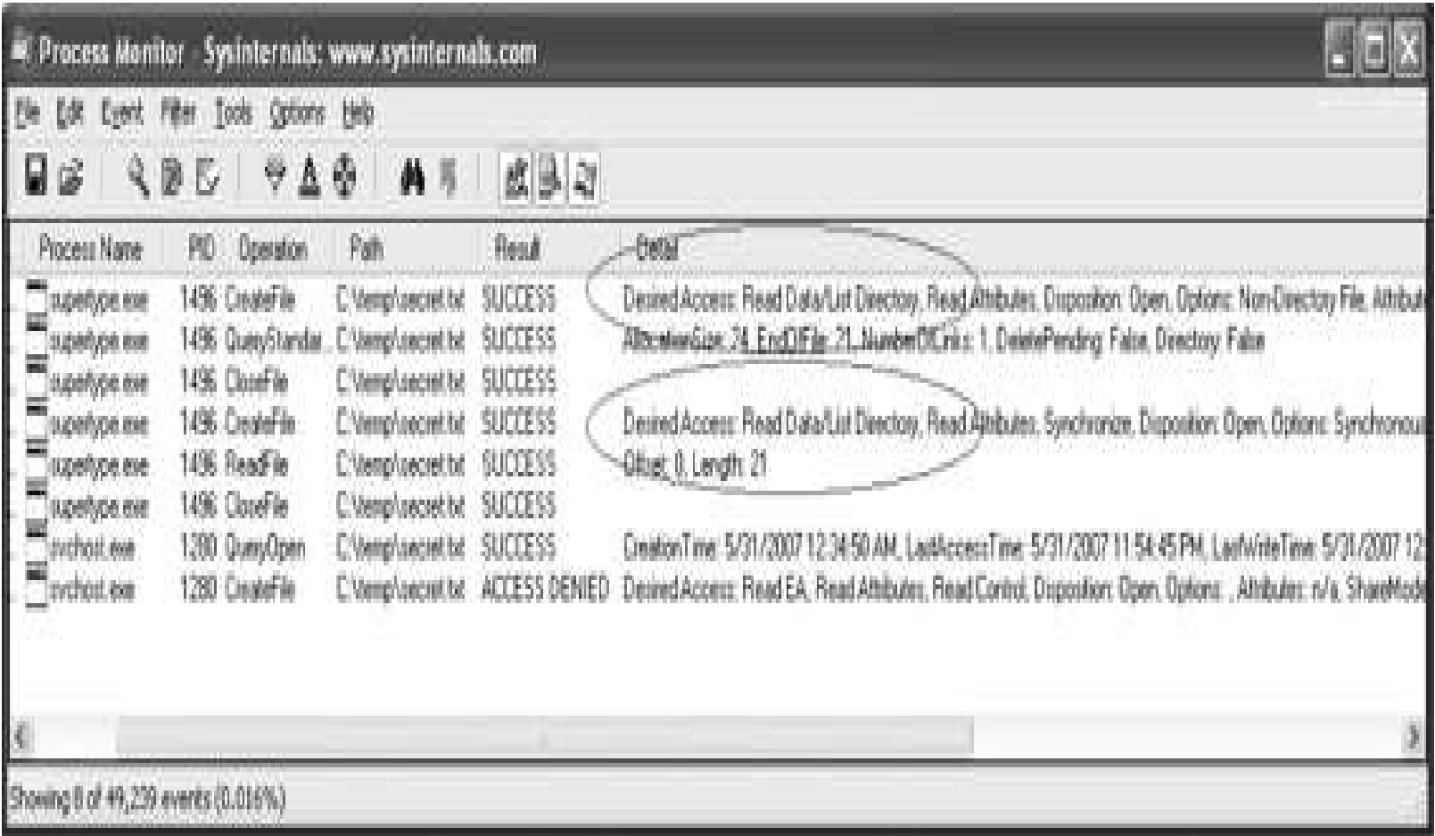
Figure 14-22 Process Monitor log of supertype.exe
