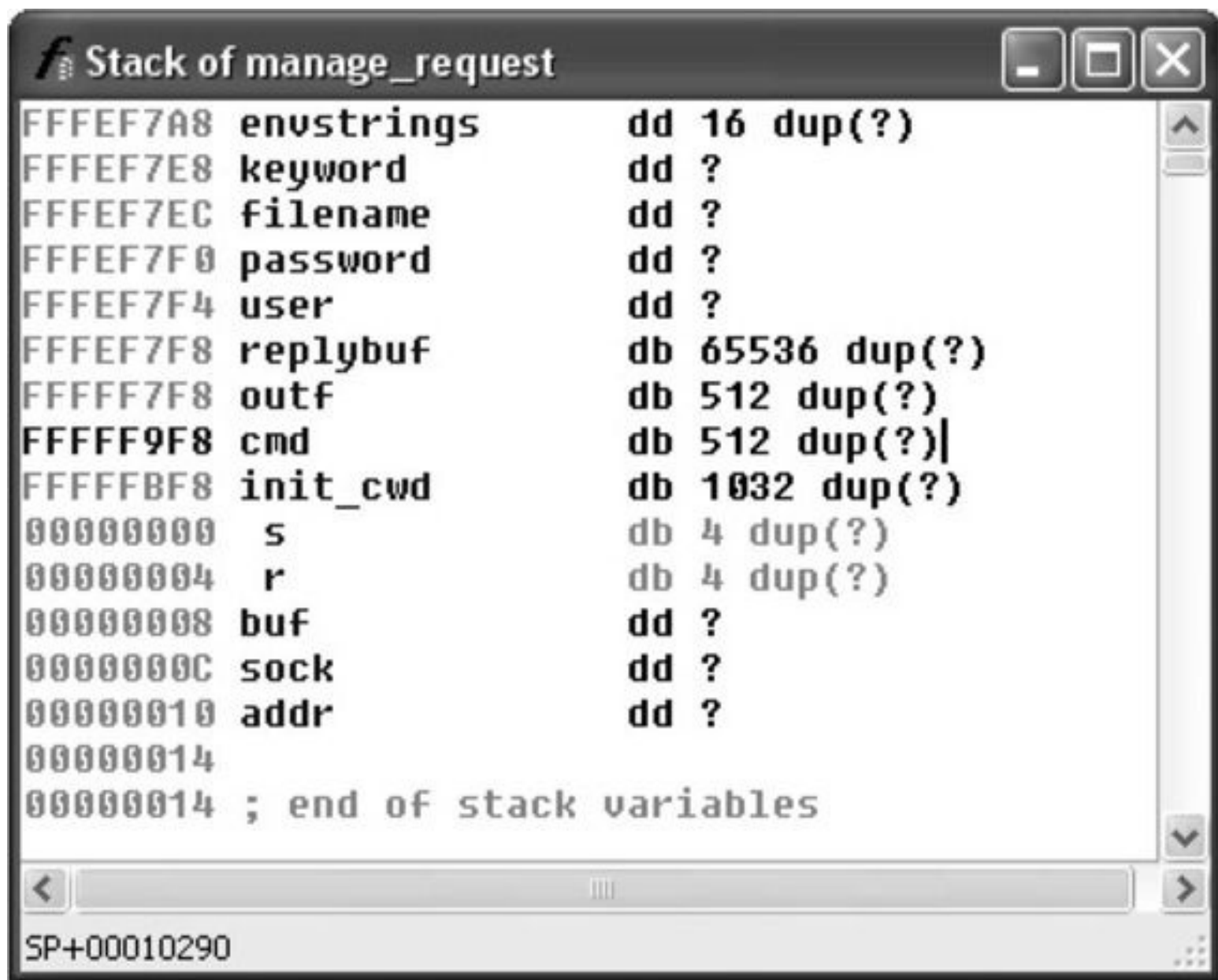
Figure 3-9 The relevant stack arguments for sprintf()
