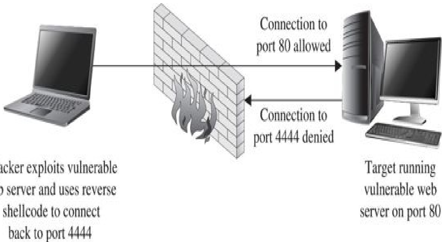
Figure 6-4 Firewall configuration that prevents reverse connecting shellcode
