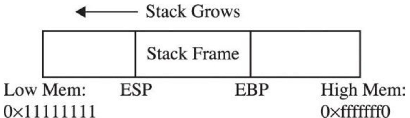
Figure 10-1 The relationship of EBP and ESP on a stack
