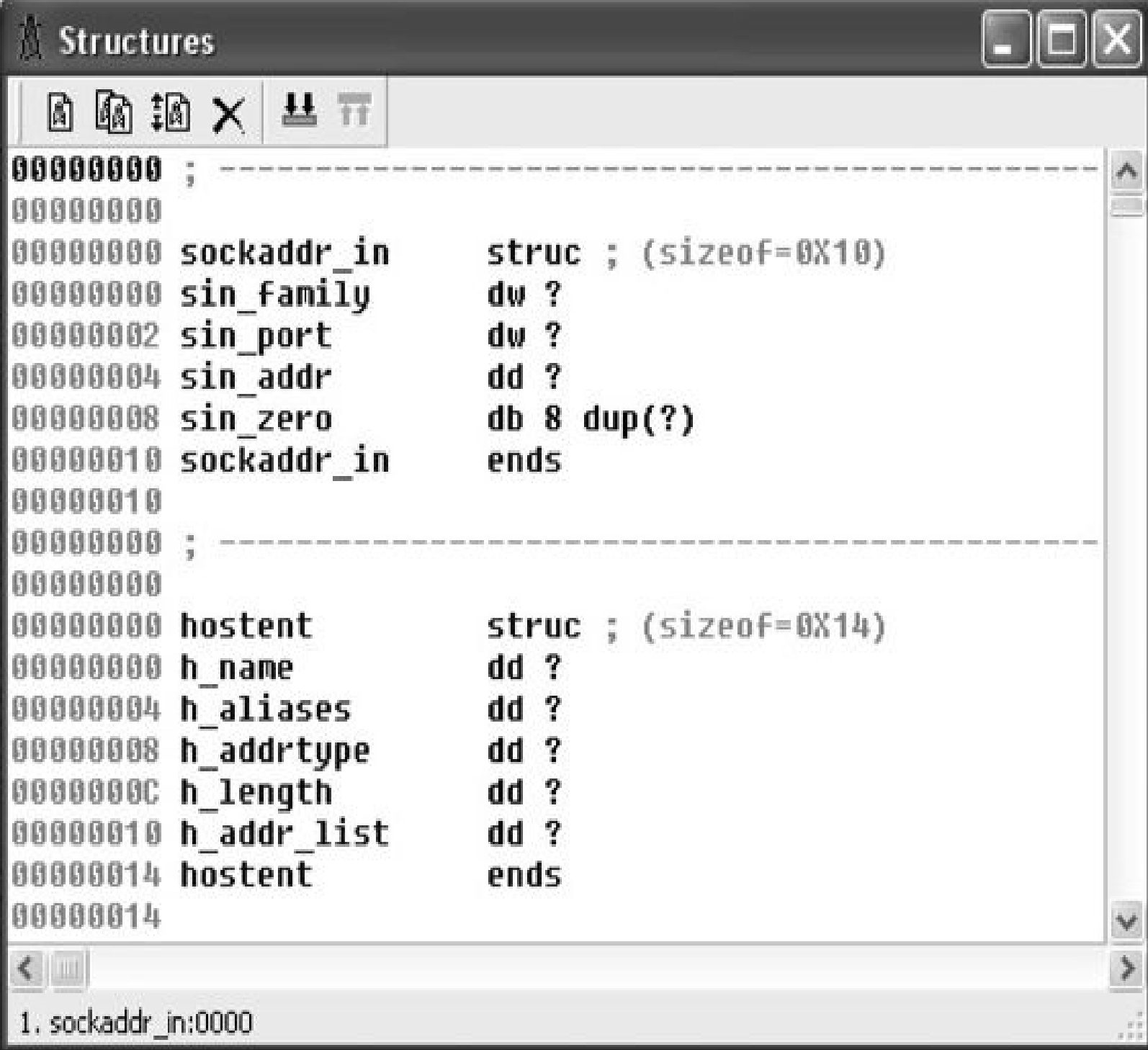
Figure 3-6 IDA Pro Structures definition window
